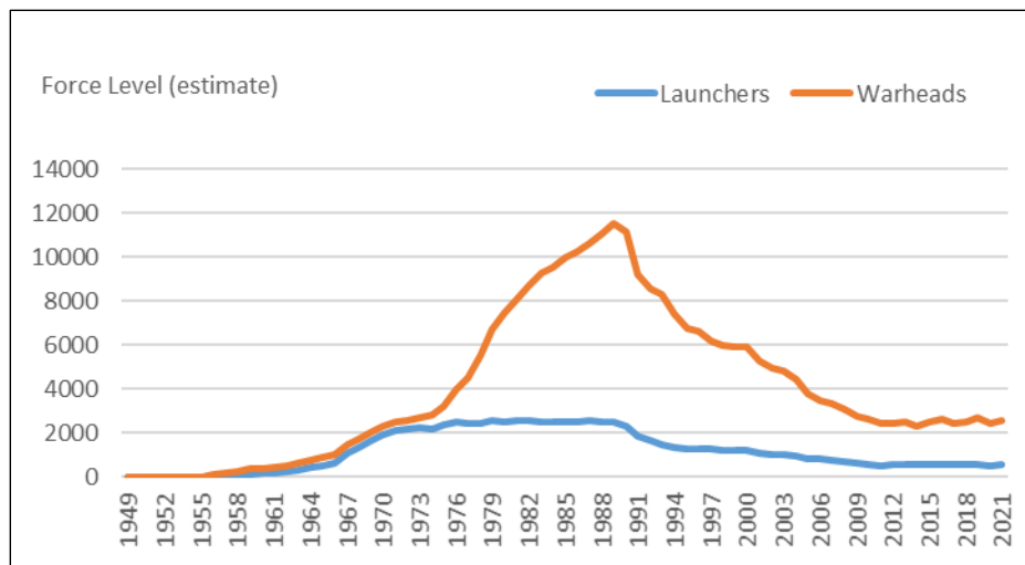
Figure 1. Estimates of Soviet/Russian Strategic Forces
